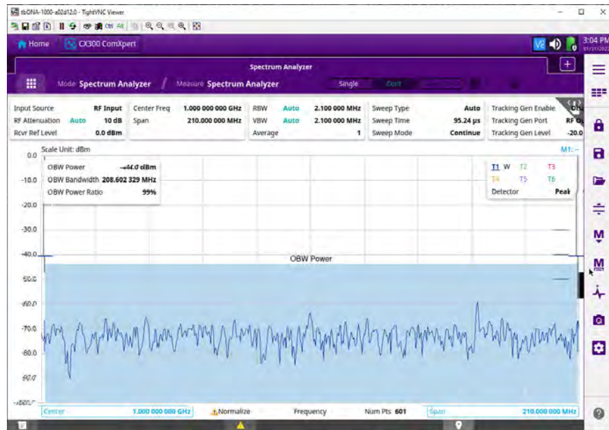
Figure 5-7 Spectrum Analyzer Screen
