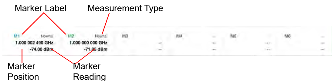
Figure 5-4 Marker Controls Toolbar
