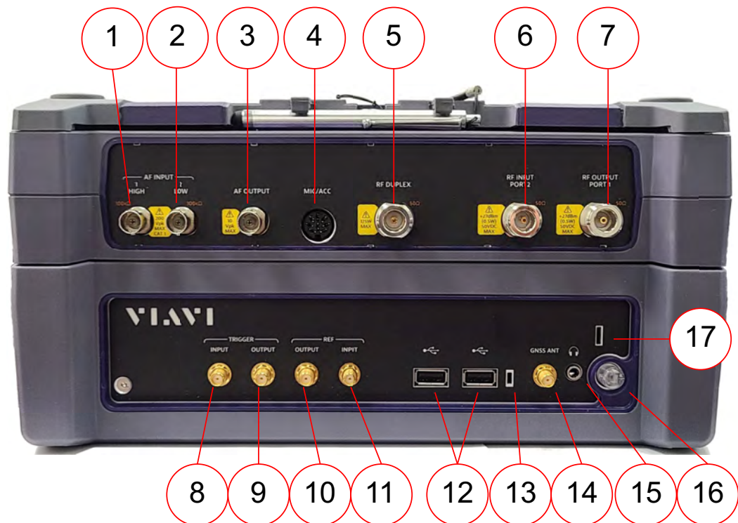
Figure 1-2 CX300 Top Panel Controls and Connectors
