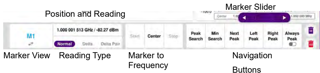
Figure 5-3 Marker Controls Toolbar
