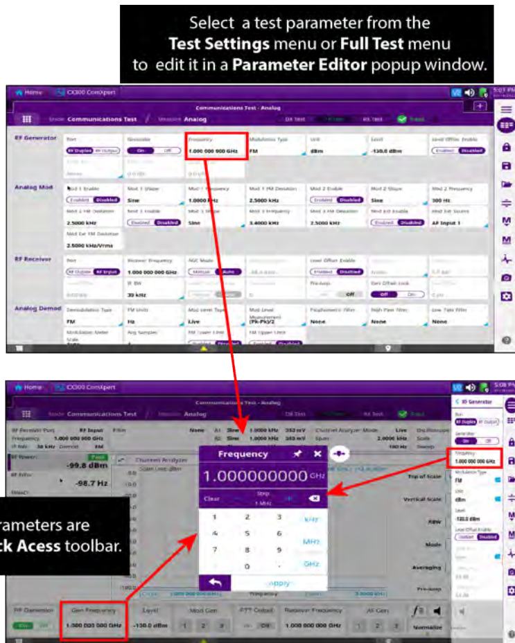
Figure 5-16 Parameter Editor & Quick Access toolbar
