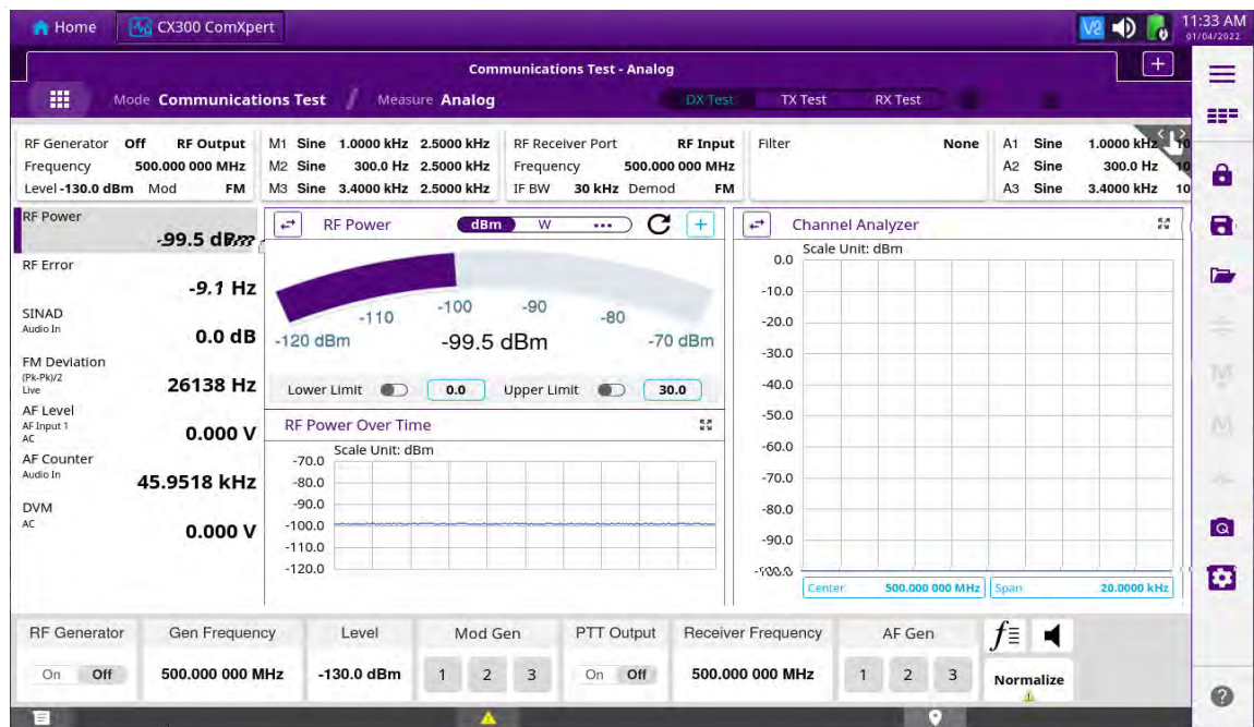
Figure 2-3 CX300 Screen Layout
